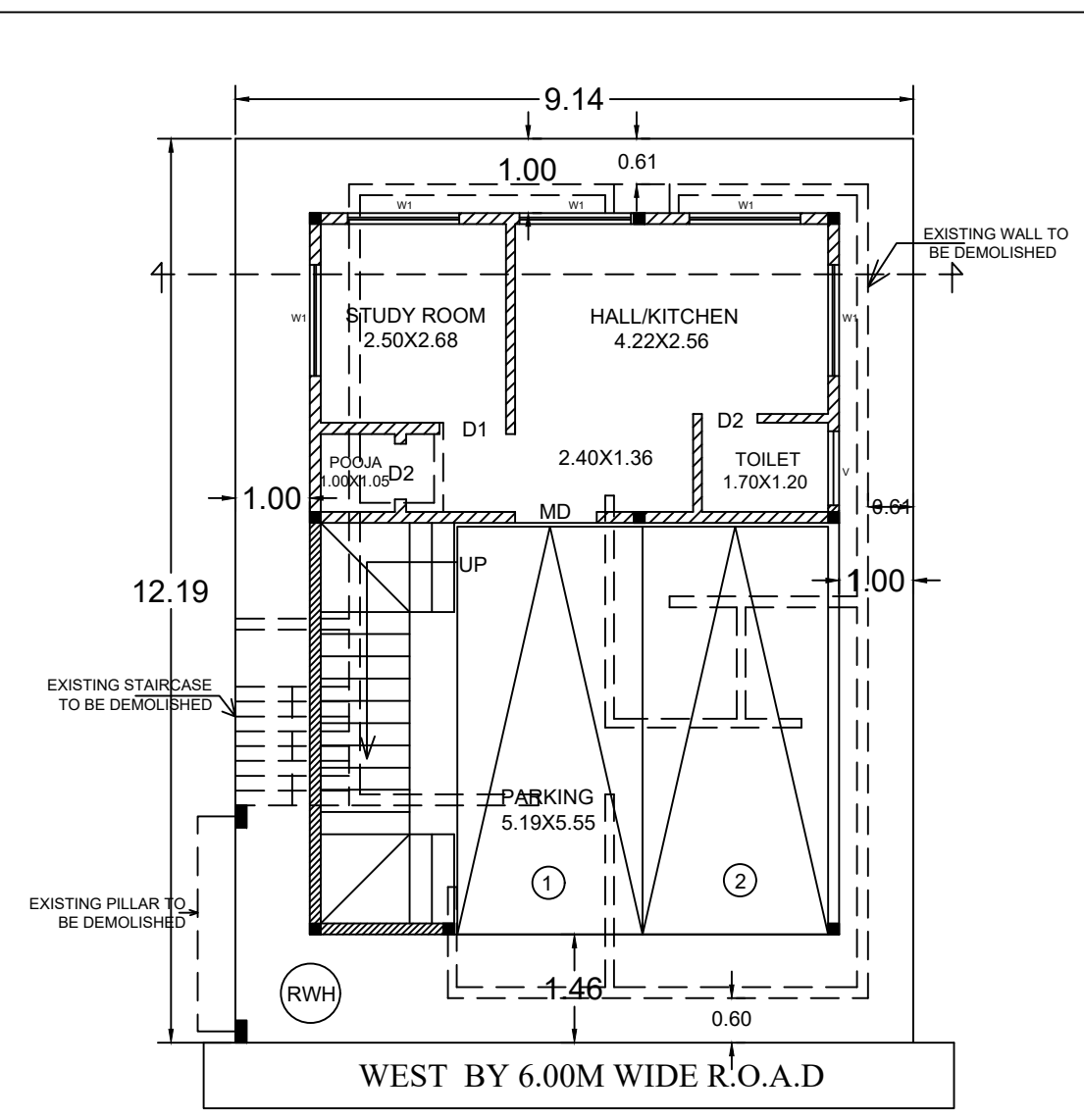
ALTERATION IN EXISTING GROUND FLOOR PLAN
